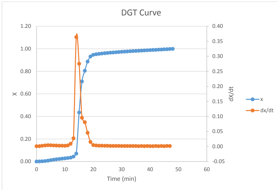
Figure 10. Differential Thermogravimetric curve.
