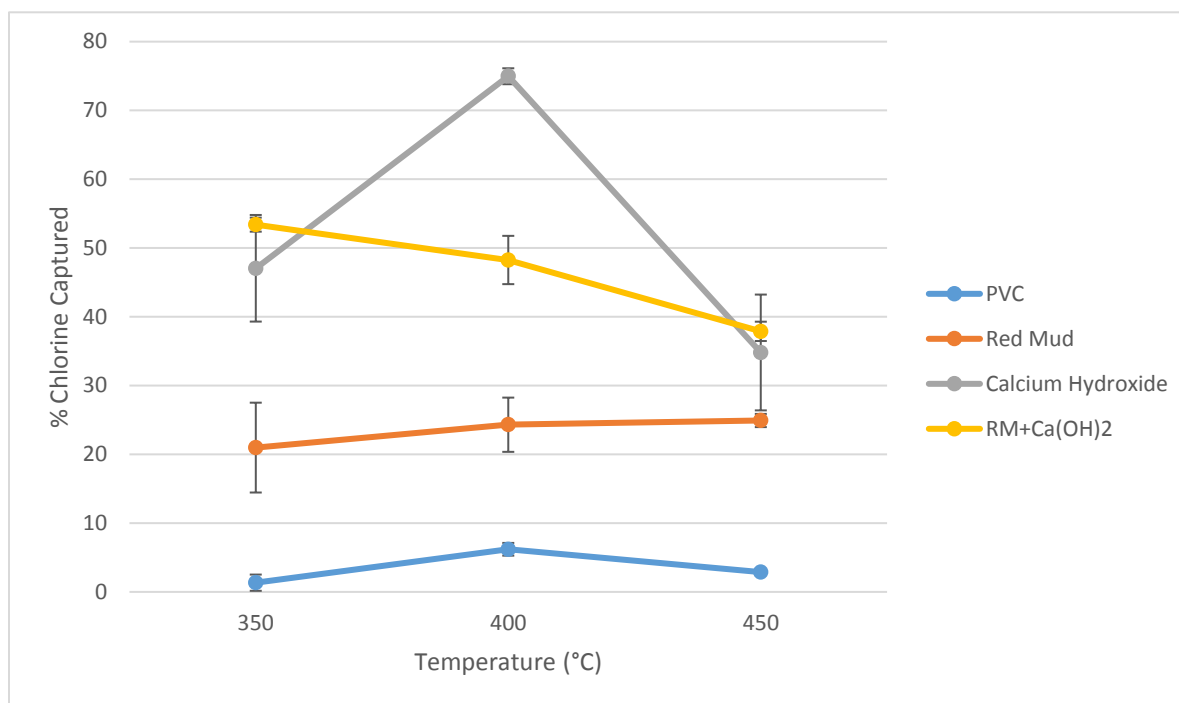
Figure 8. Temperature Dependence on Chlorine Adsorption. The error bars are the standard deviation.
