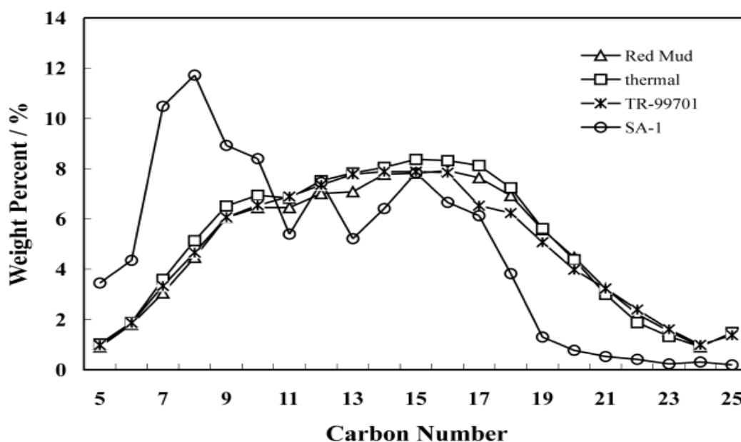
Figure 4. Carbon Number Probability graph (C-NP gram) from thermal and catalytic degradation of PE/PVC at 430 °C. Adapted from (Yanik, et al. 2001).
